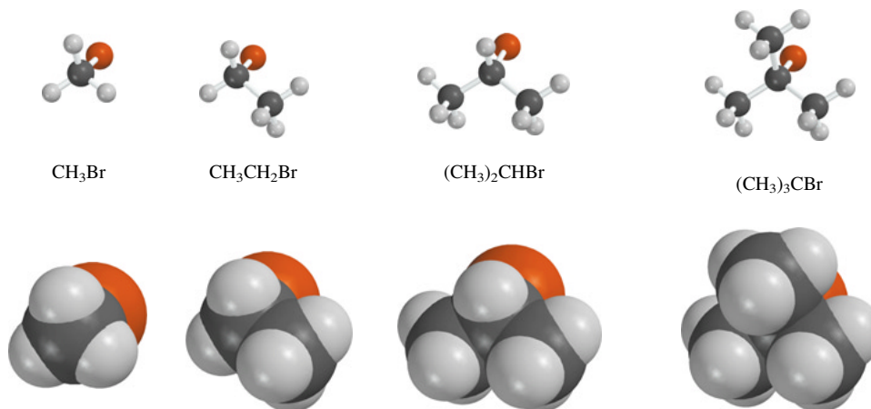
FIGURE 8.3 Ball-and-spoke and space-filling models of alkyl bromides, showing how substituents shield the carbon atom that bears the leaving group from attack by a nucleophile. The nucleophile must attack from the side opposite the bond to the leaving group.
